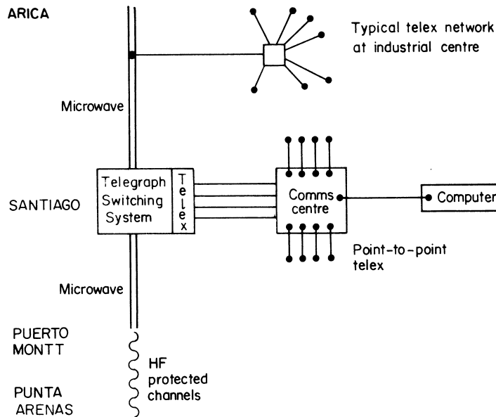
Figure 2. Nature of Telecommunications using existing public system. This cannot yet accept even low speed data. System uses Alphabet No. 2 at 50 Bauds.
